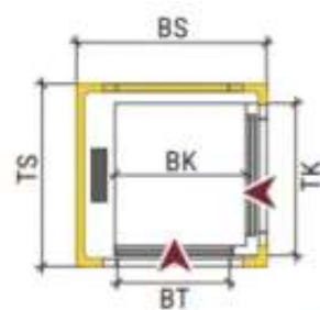
90° CAR ENTRANCES (2 x 90°)
