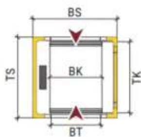
THROUGH CAR ENTRANCES (2 x 180°)
