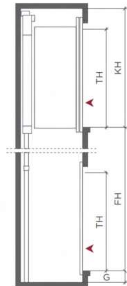
VERTICAL SECTION
